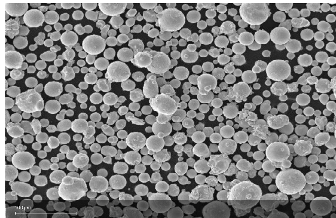
SEM of EOS NickelAlloy IN939 powder.
